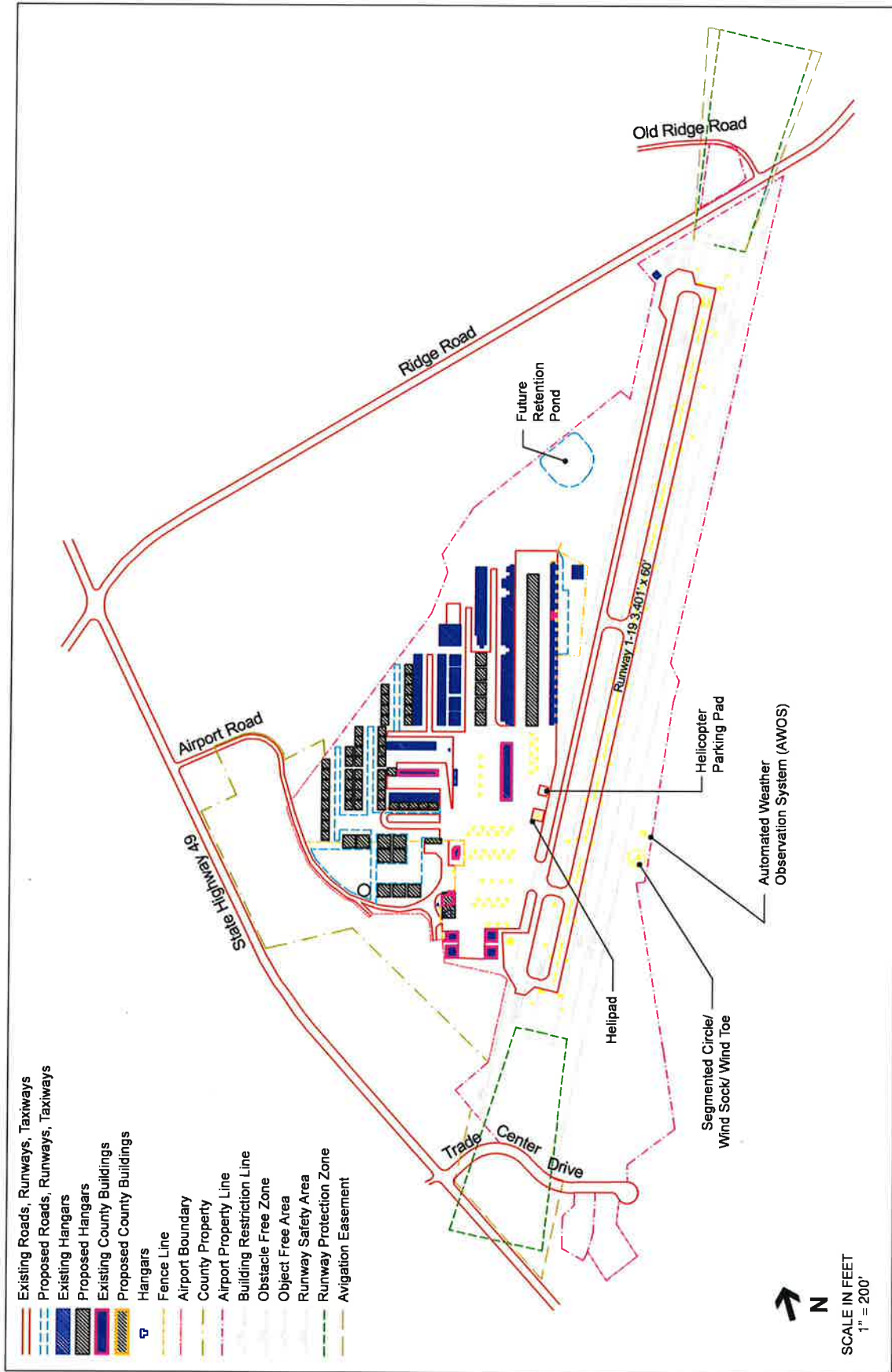
Amador County Westover Field ALUCP - 2/11/96 Figure 2-2 Airport Layout Plan
